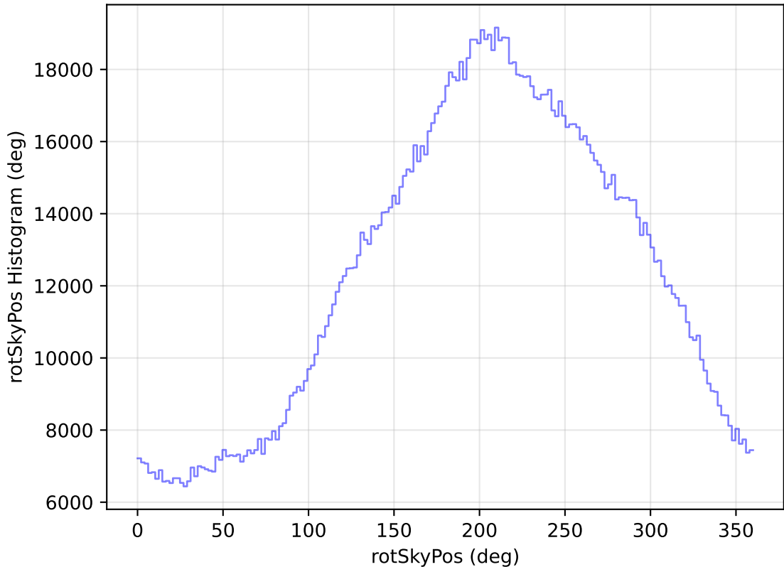
too_elab_heavy_r64_d2_griz_v3.4_10yrs All sky all bands: rotSkyPos Histogram
