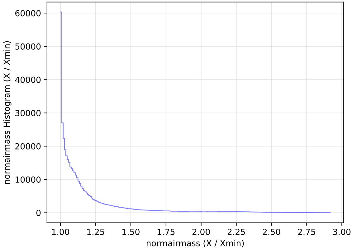
too_elab_heavy_r64_d2_griz_v3.4_10yrs WFD z band: normairmass Histogram
