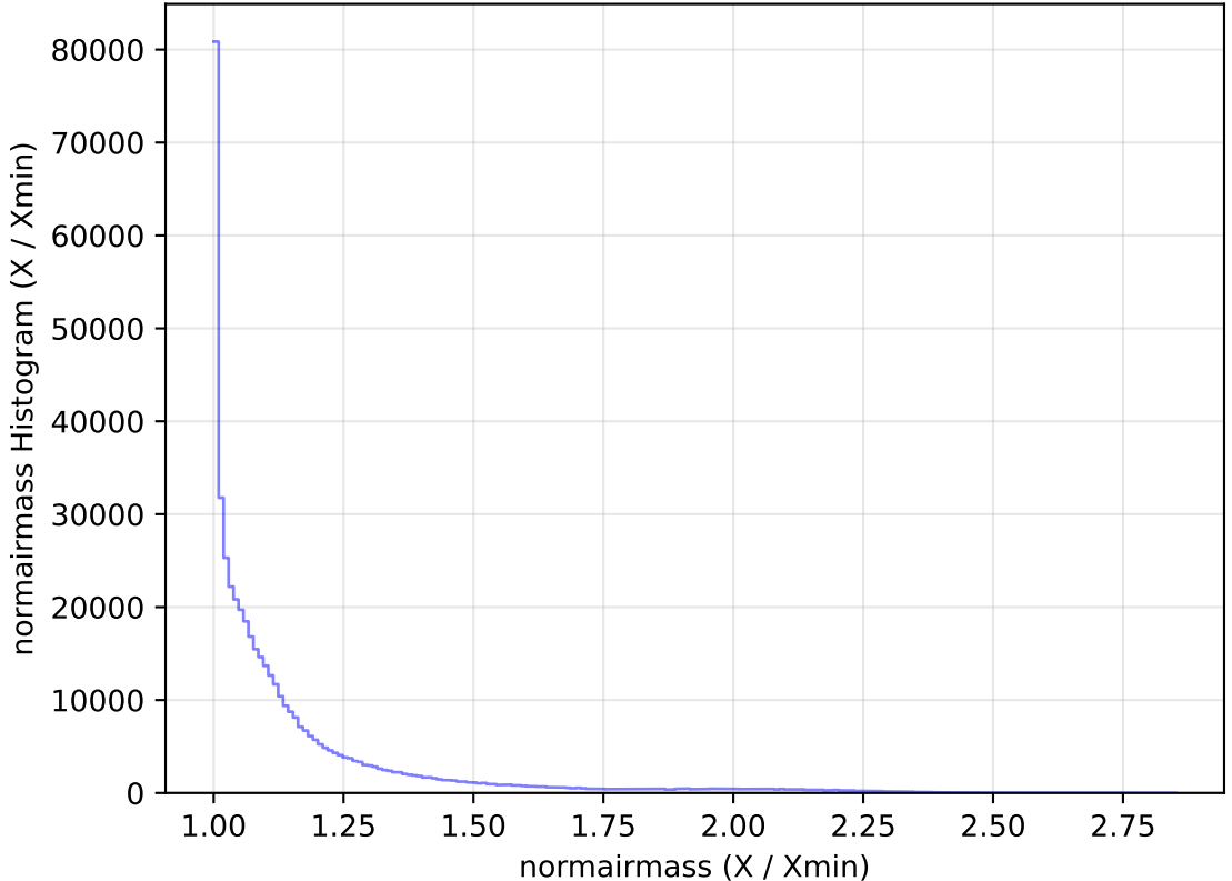
too_elab_heavy_r64_d2_griz_v3.4_10yrs WFD r band: normairmass Histogram
