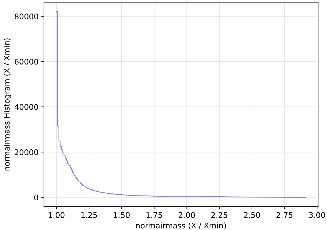
too_elab_heavy_r64_d2_griz_v3.4_10yrs WFD i band: normairmass Histogram
