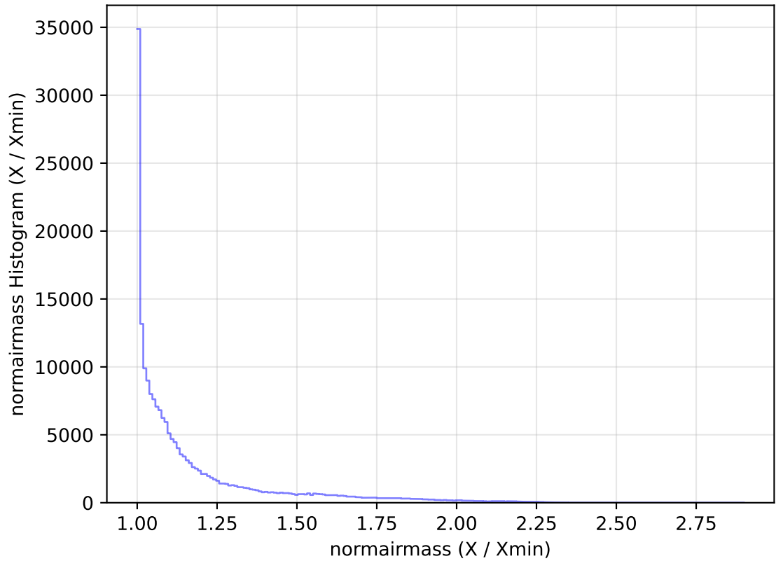
too_elab_heavy_r64_d2_griz_v3.4_10yrs WFD g band: normairmass Histogram
