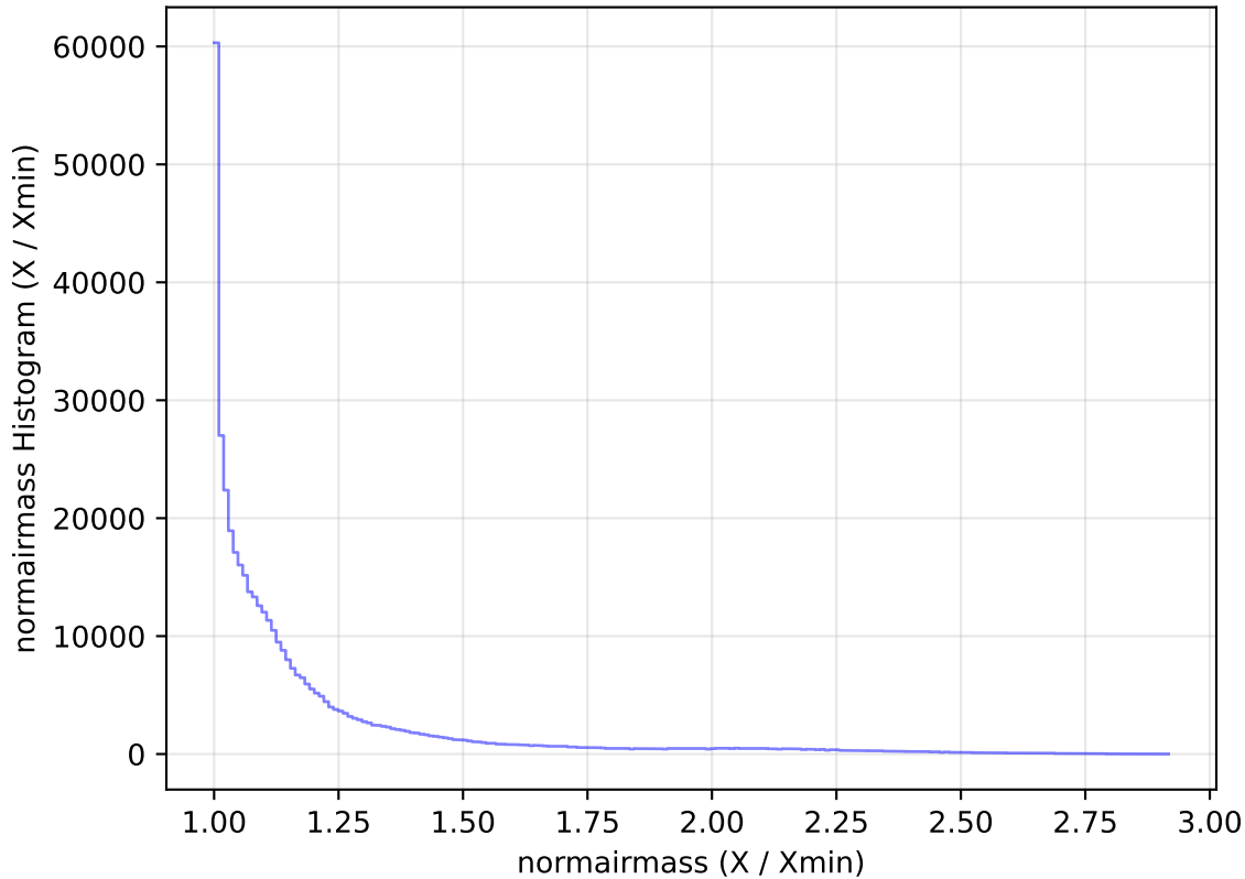
too_elab_heavy_r64_d2_griz_v3.4_10yrs All sky z band: normairmass Histogram
