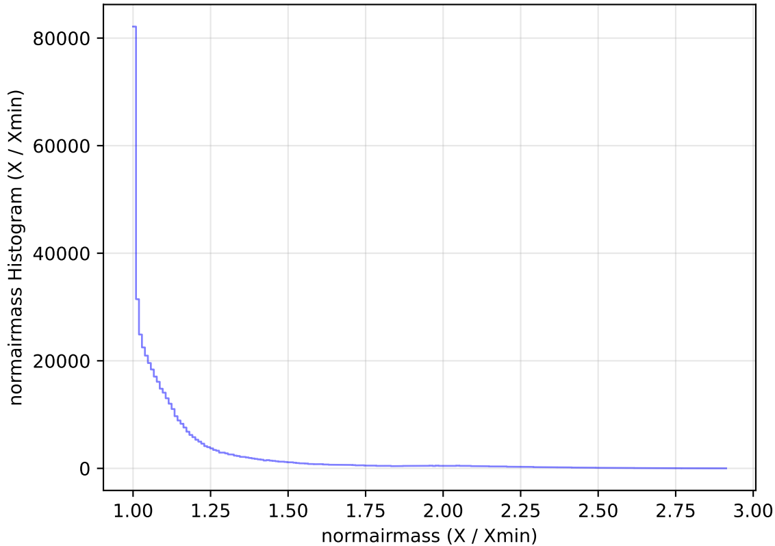
too_elab_heavy_r64_d2_griz_v3.4_10yrs All sky i band: normairmass Histogram
