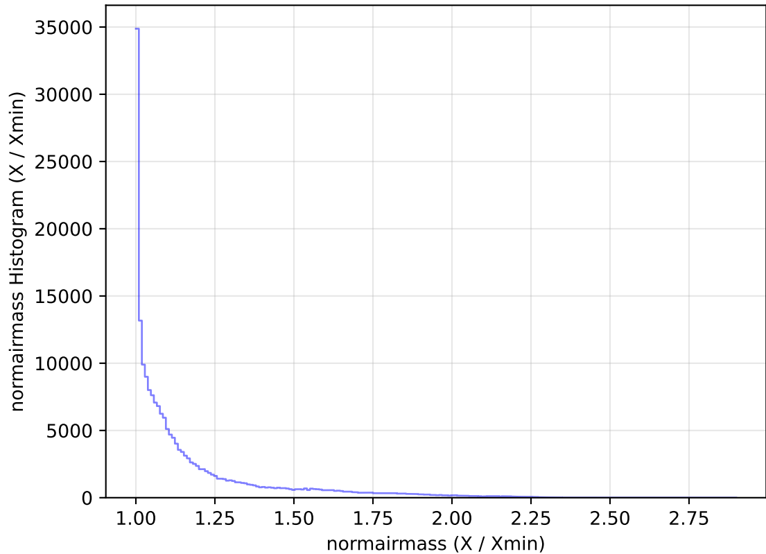
too_elab_heavy_r64_d2_griz_v3.4_10yrs All sky g band: normairmass Histogram
