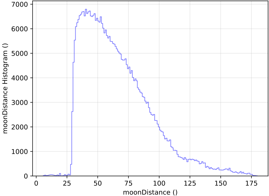
too_elab_heavy_r64_d2_griz_v3.4_10yrs WFD y band: moonDistance Histogram
