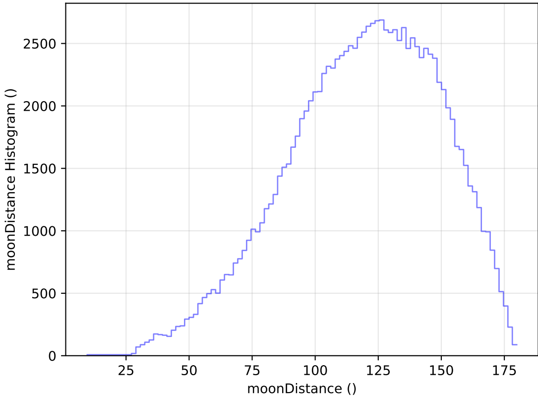
too_elab_heavy_r64_d2_griz_v3.4_10yrs WFD u band: moonDistance Histogram
