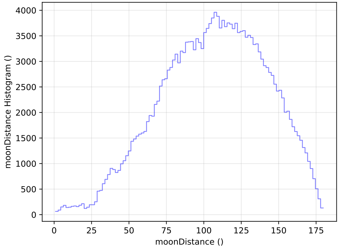
too_elab_heavy_r64_d2_griz_v3.4_10yrs WFD g band: moonDistance Histogram
