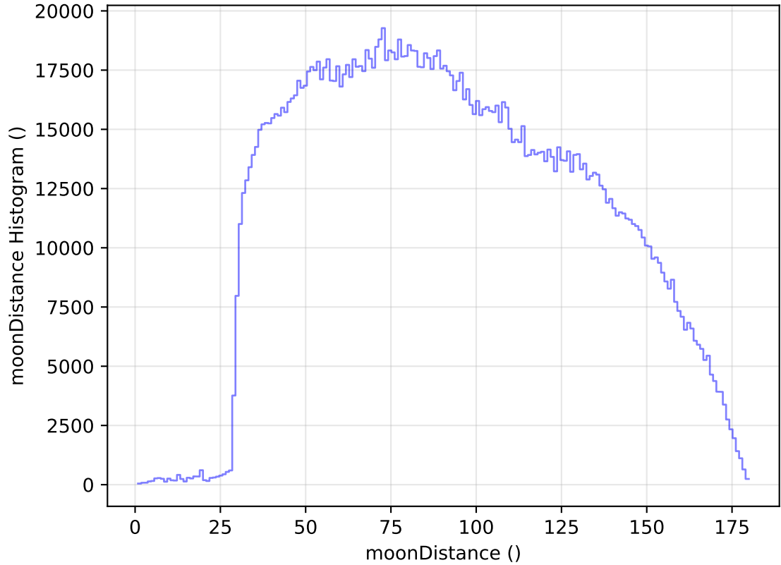
too_elab_heavy_r64_d2_griz_v3.4_10yrs WFD all bands: moonDistance Histogram
