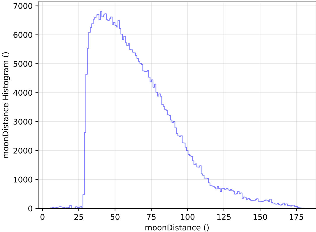
too_elab_heavy_r64_d2_griz_v3.4_10yrs All sky y band: moonDistance Histogram
