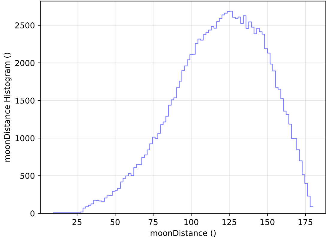
too_elab_heavy_r64_d2_griz_v3.4_10yrs All sky u band: moonDistance Histogram
