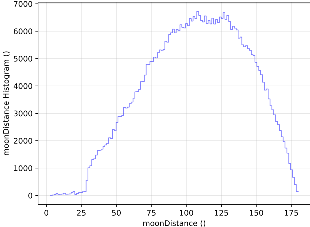
too_elab_heavy_r64_d2_griz_v3.4_10yrs All sky r band: moonDistance Histogram
