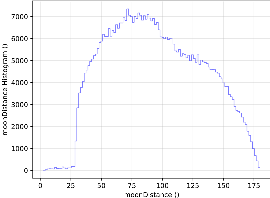
too_elab_heavy_r64_d2_griz_v3.4_10yrs All sky i band: moonDistance Histogram
