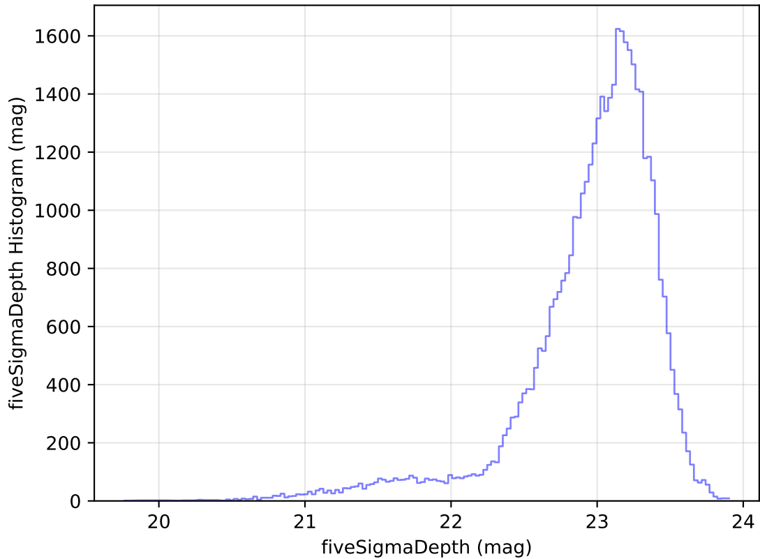
too_elab_heavy_r64_d2_griz_v3.4_10yrs Yr 1 z band: fiveSigmaDepth Histogram
