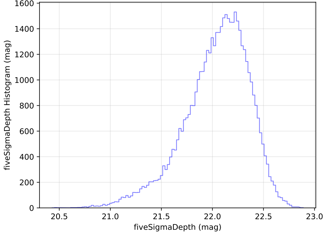
too_elab_heavy_r64_d2_griz_v3.4_10yrs Yr 1 y band: fiveSigmaDepth Histogram
