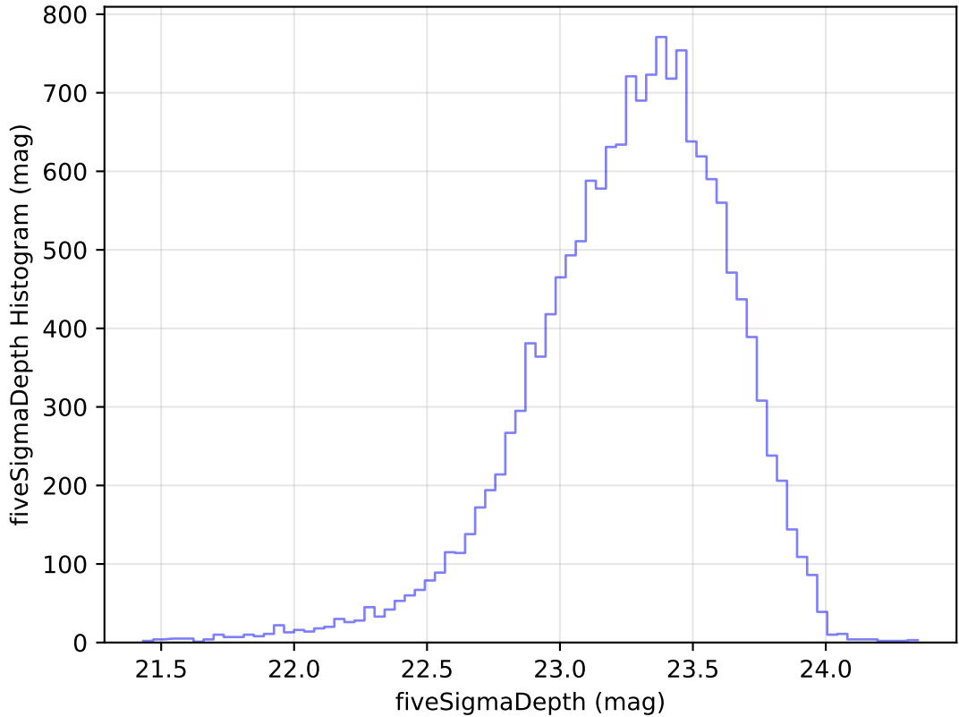
too_elab_heavy_r64_d2_griz_v3.4_10yrs Yr 1 u band: fiveSigmaDepth Histogram
