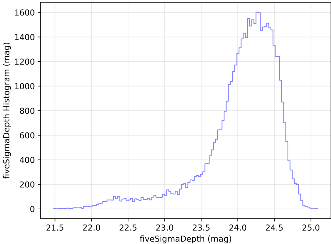
too_elab_heavy_r64_d2_griz_v3.4_10yrs Yr 1 r band: fiveSigmaDepth Histogram
