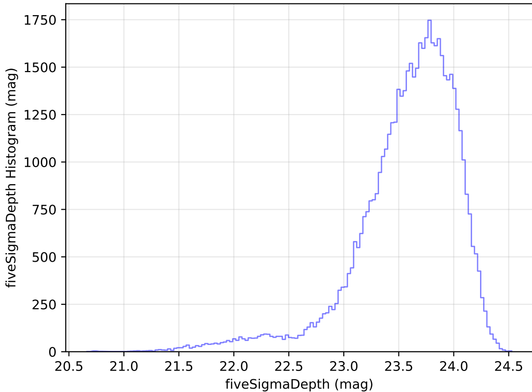
too_elab_heavy_r64_d2_griz_v3.4_10yrs Yr 1 i band: fiveSigmaDepth Histogram
