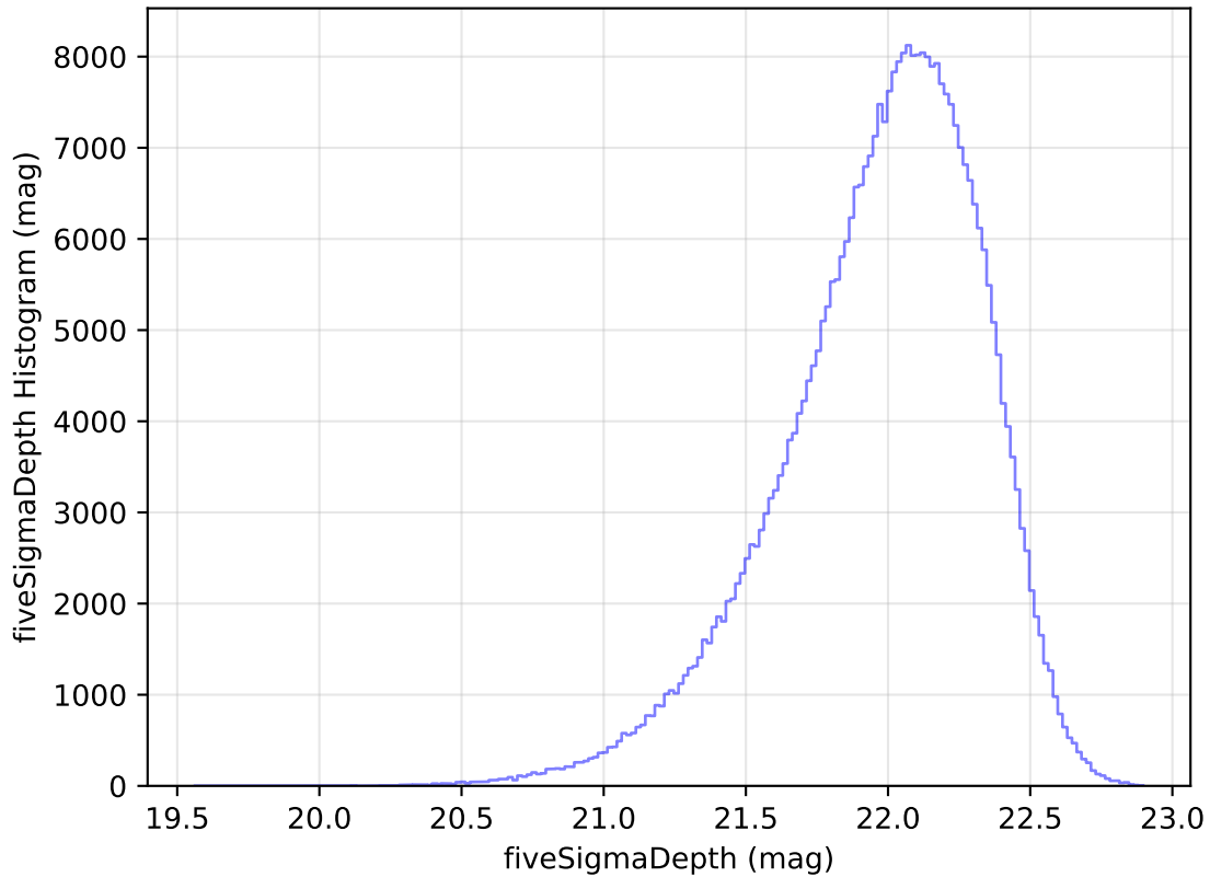
too_elab_heavy_r64_d2_griz_v3.4_10yrs WFD y band: fiveSigmaDepth Histogram
