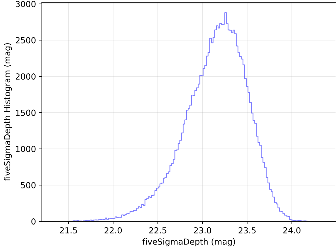
too_elab_heavy_r64_d2_griz_v3.4_10yrs WFD u band: fiveSigmaDepth Histogram
