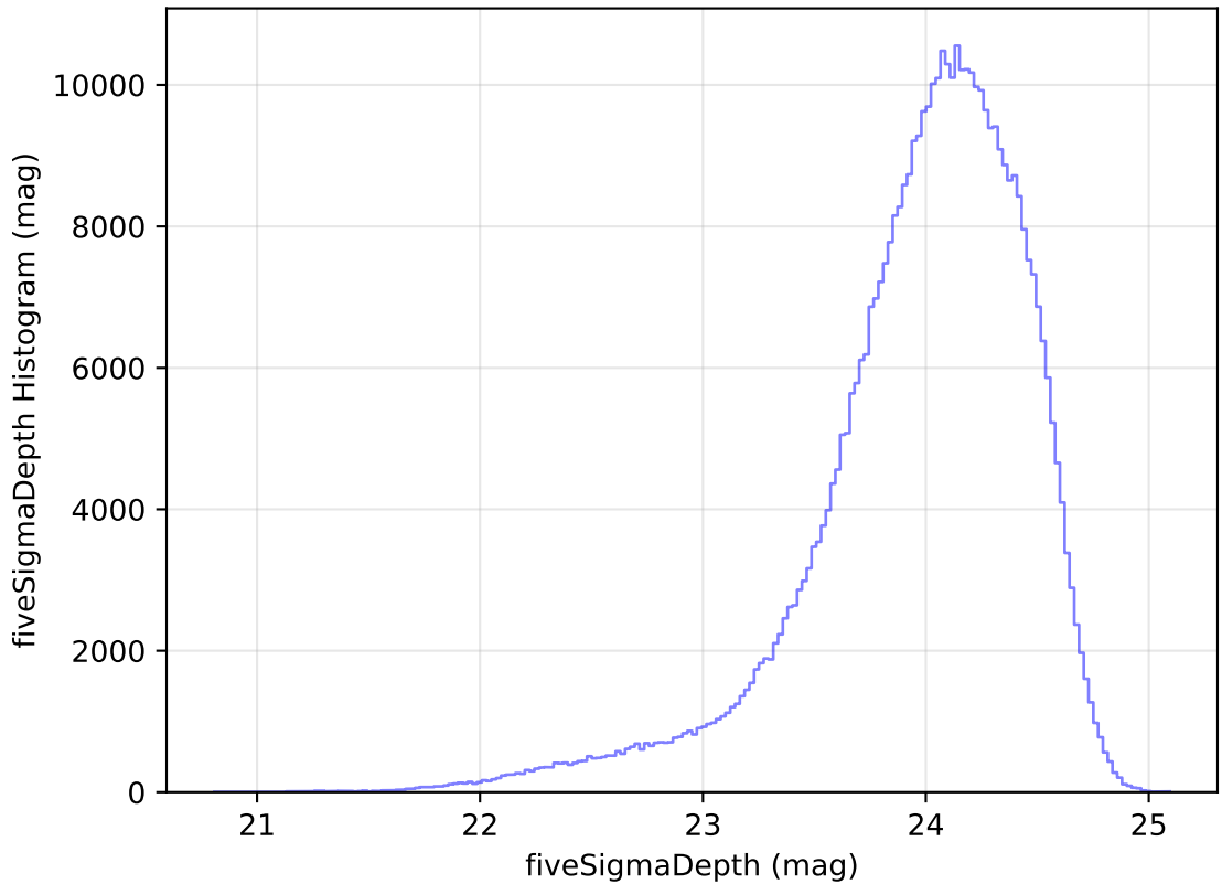
too_elab_heavy_r64_d2_griz_v3.4_10yrs WFD r band: fiveSigmaDepth Histogram
