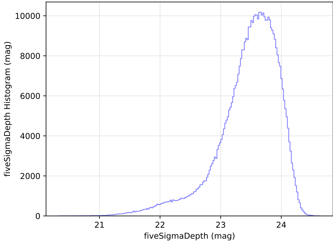
too_elab_heavy_r64_d2_griz_v3.4_10yrs WFD i band: fiveSigmaDepth Histogram
