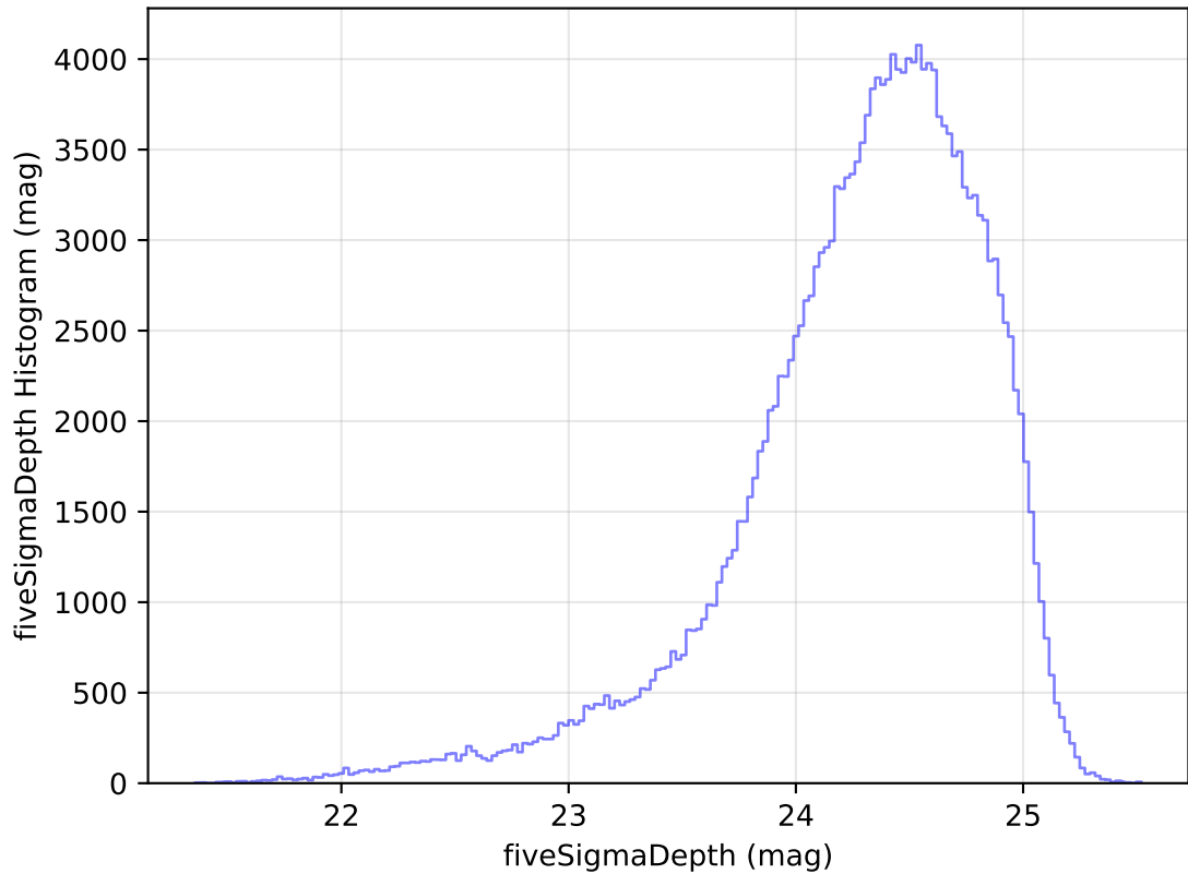
too_elab_heavy_r64_d2_griz_v3.4_10yrs WFD g band: fiveSigmaDepth Histogram
