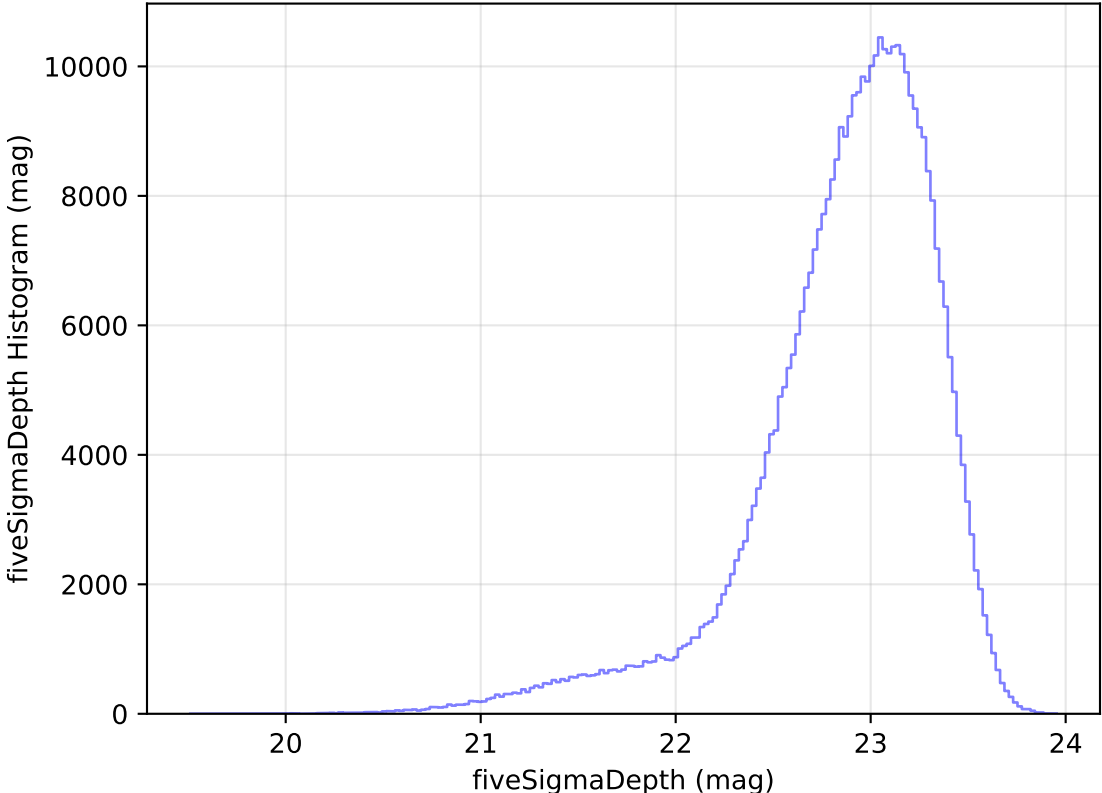
too_elab_heavy_r64_d2_griz_v3.4_10yrs All sky z band: fiveSigmaDepth Histogram
