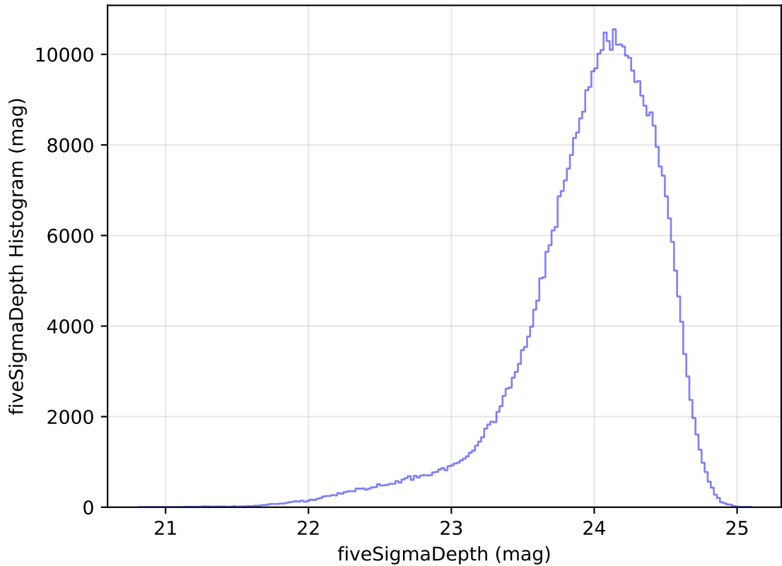
too_elab_heavy_r64_d2_griz_v3.4_10yrs All sky r band: fiveSigmaDepth Histogram
