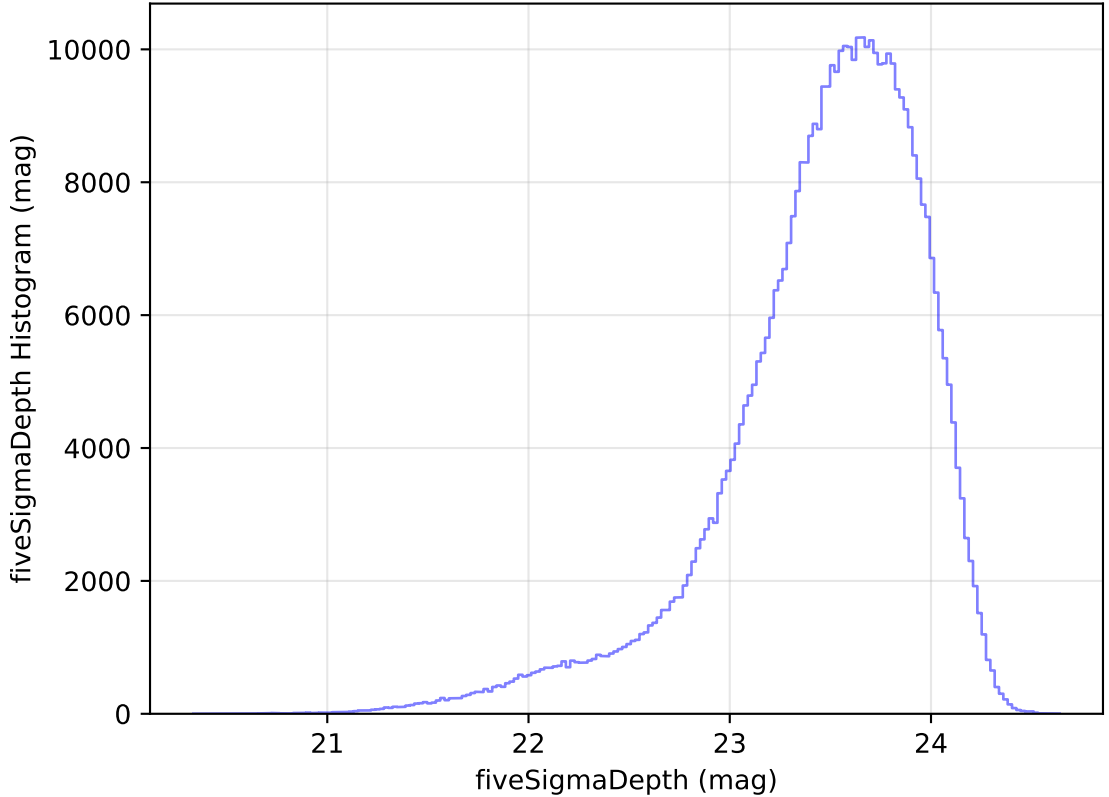
too_elab_heavy_r64_d2_griz_v3.4_10yrs All sky i band: fiveSigmaDepth Histogram
