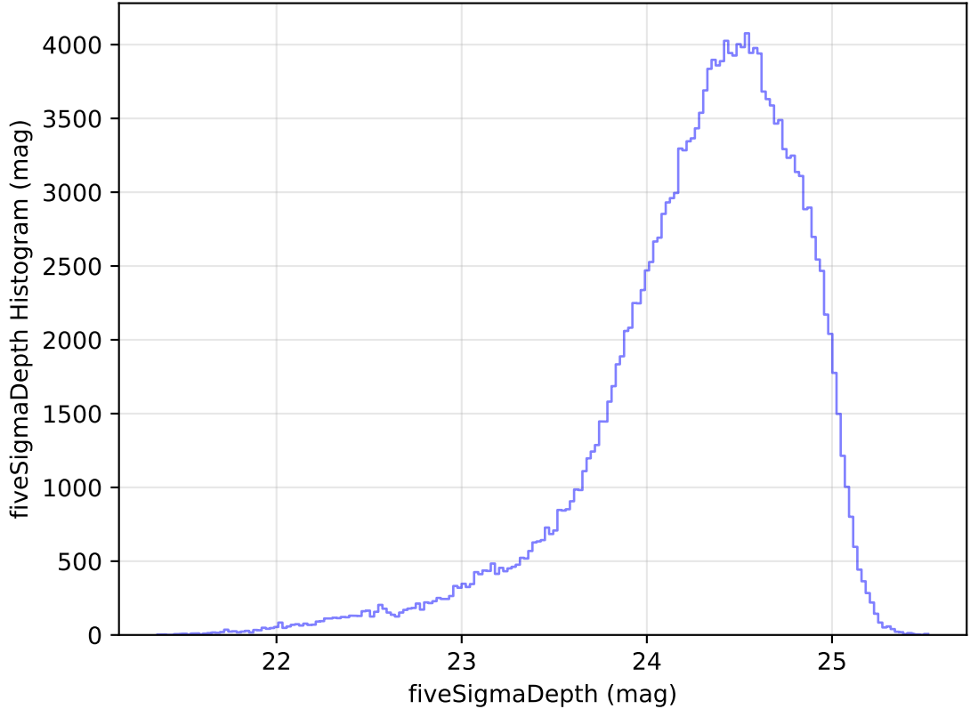
too_elab_heavy_r64_d2_griz_v3.4_10yrs All sky g band: fiveSigmaDepth Histogram
