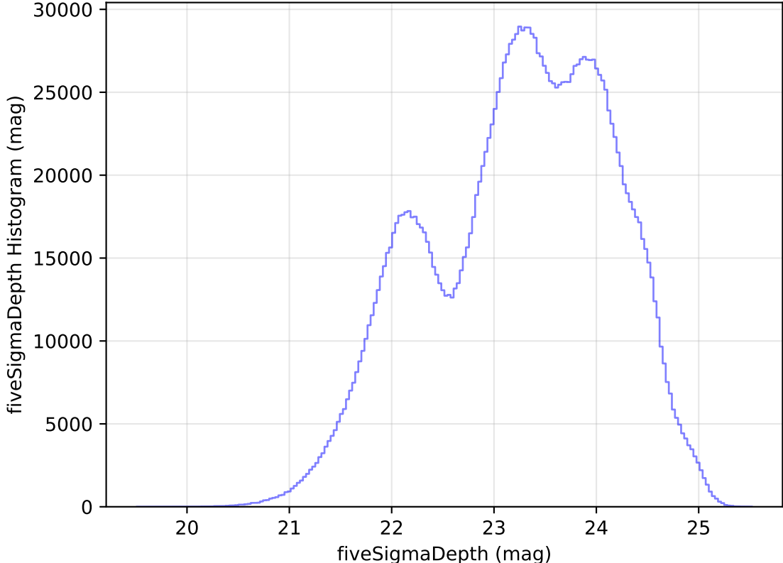
too_elab_heavy_r64_d2_griz_v3.4_10yrs All sky all bands: fiveSigmaDepth Histogram
