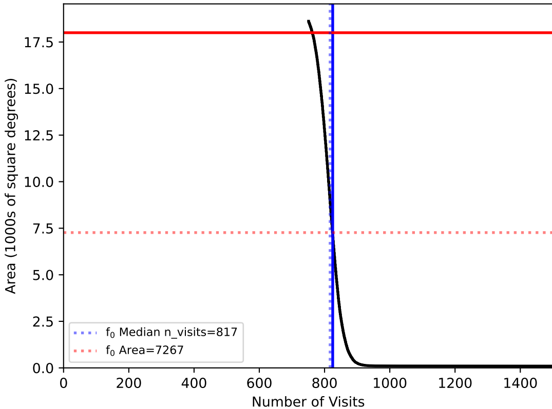
too_elab_heavy_r64_d2_griz_v3.4_10yrs WFD: f0
