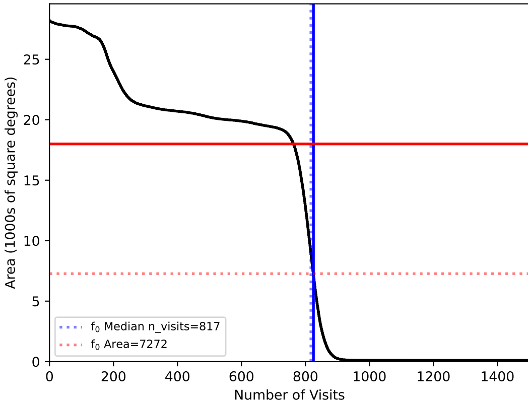
too_elab_heavy_r64_d2_griz_v3.4_10yrs All sky: f0
