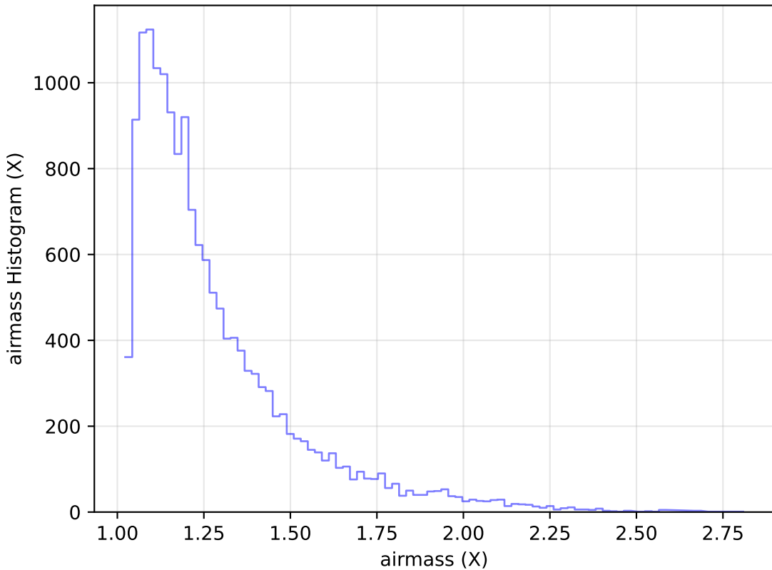
too_elab_heavy_r64_d2_griz_v3.4_10yrs Yr 1 u band: airmass Histogram
