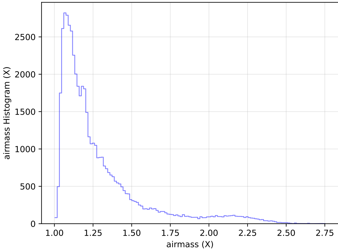
too_elab_heavy_r64_d2_griz_v3.4_10yrs Yr 1 r band: airmass Histogram
