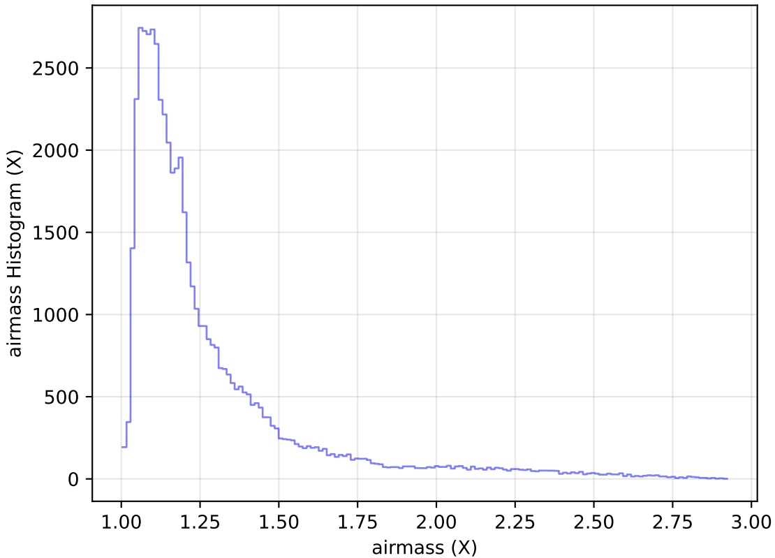
too_elab_heavy_r64_d2_griz_v3.4_10yrs Yr 1 i band: airmass Histogram
