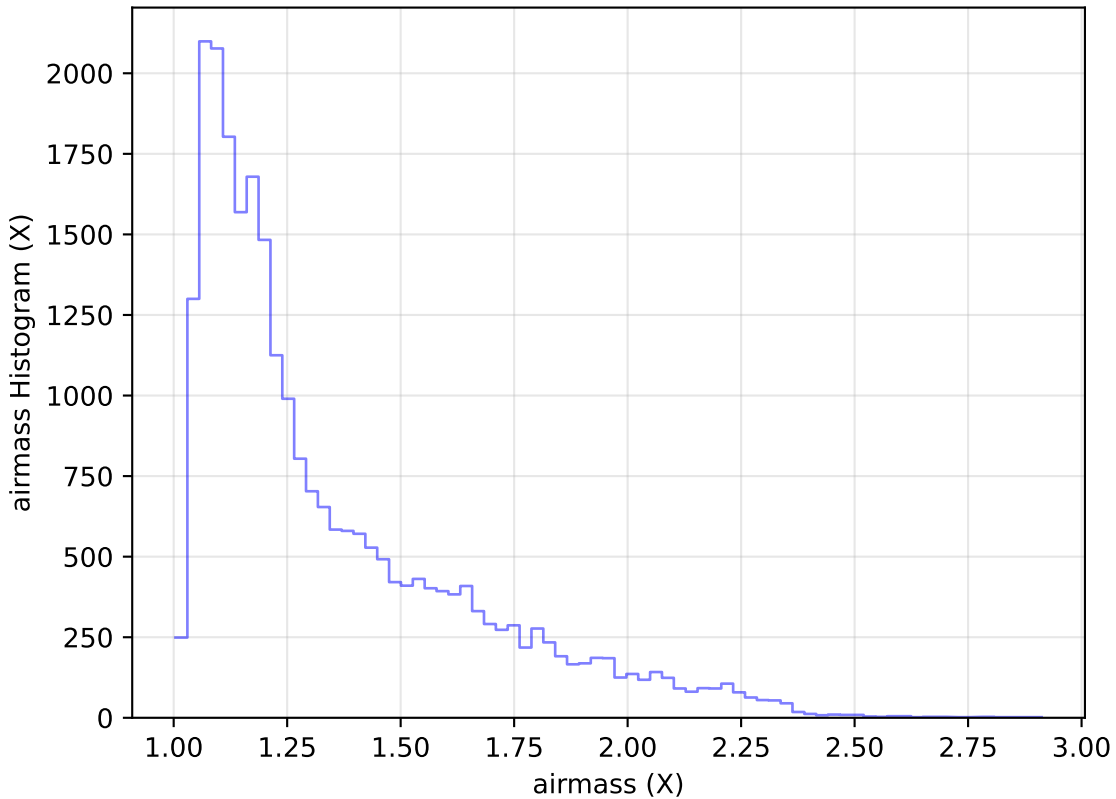
too_elab_heavy_r64_d2_griz_v3.4_10yrs Yr 1 g band: airmass Histogram
