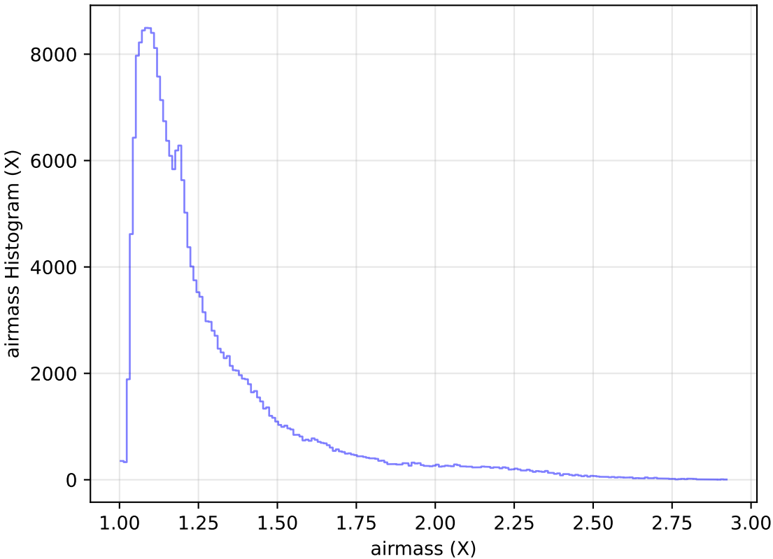
too_elab_heavy_r64_d2_griz_v3.4_10yrs Yr 1 all bands: airmass Histogram
