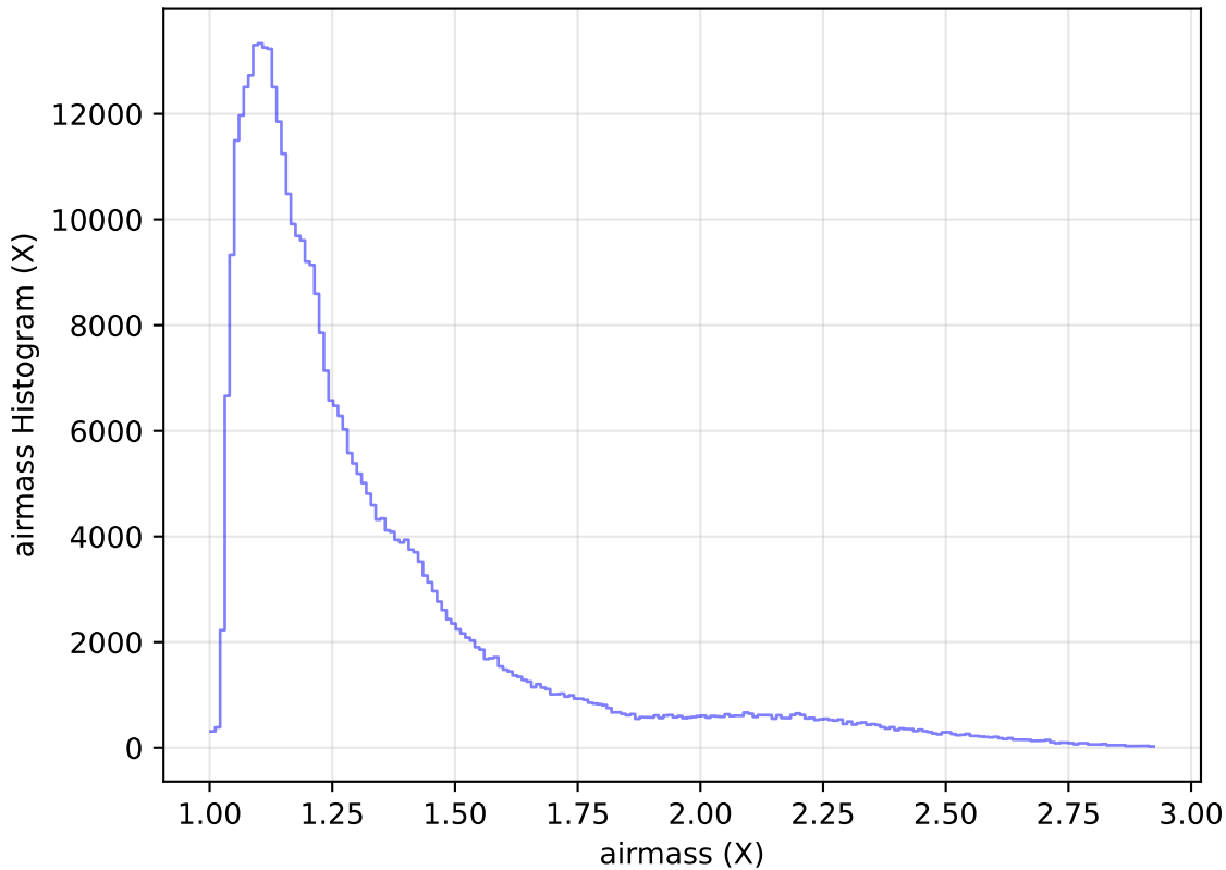
too_elab_heavy_r64_d2_griz_v3.4_10yrs WFD z band: airmass Histogram
