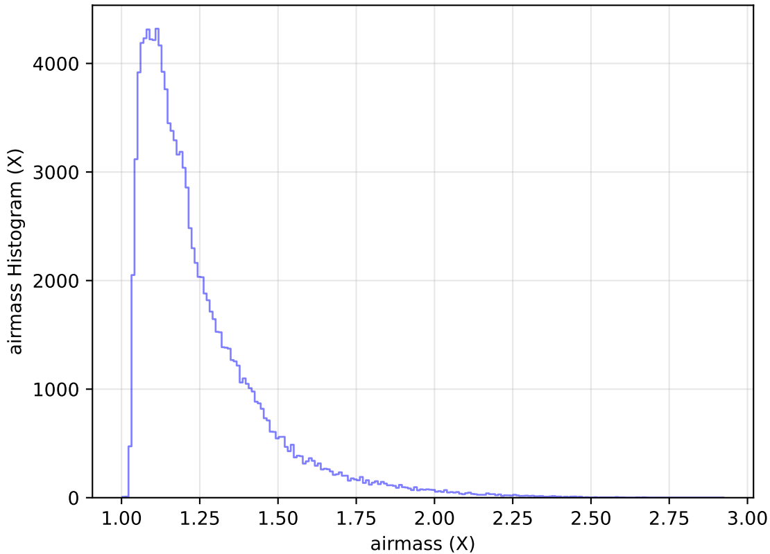
too_elab_heavy_r64_d2_griz_v3.4_10yrs WFD u band: airmass Histogram
