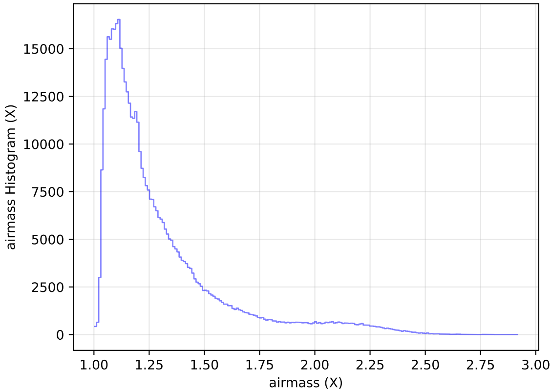
too_elab_heavy_r64_d2_griz_v3.4_10yrs WFD r band: airmass Histogram
