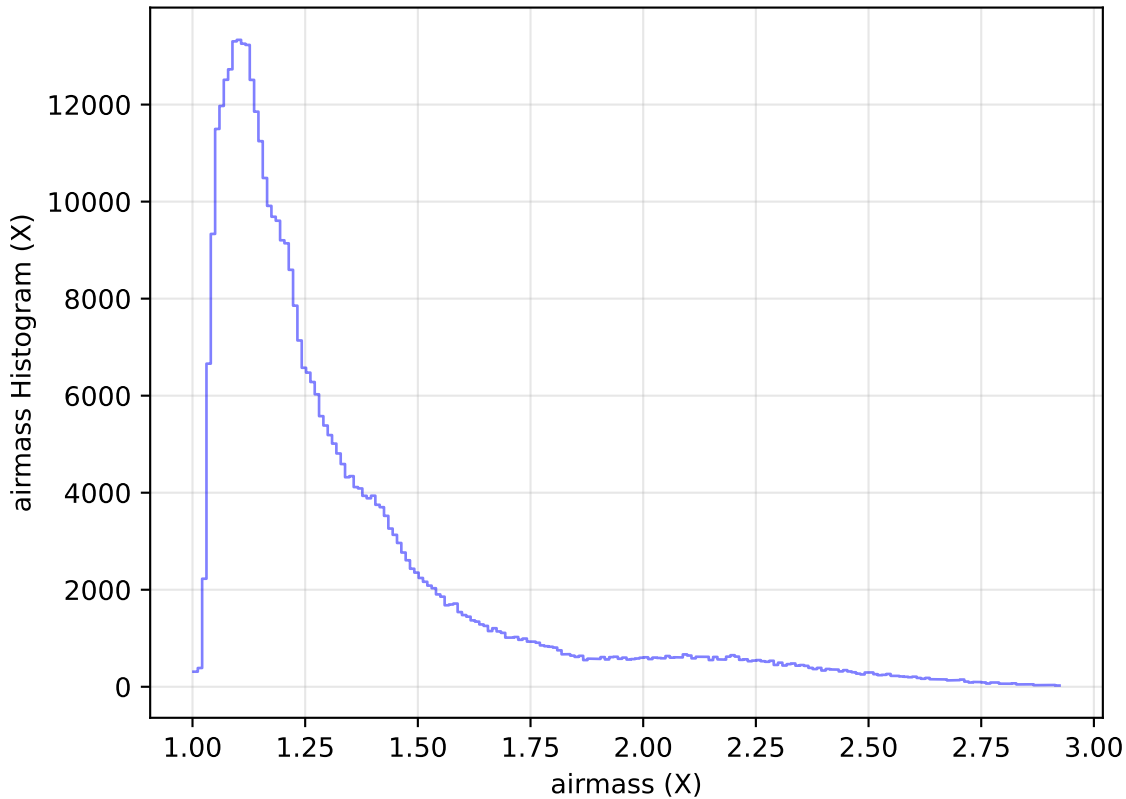
too_elab_heavy_r64_d2_griz_v3.4_10yrs All sky z band: airmass Histogram
