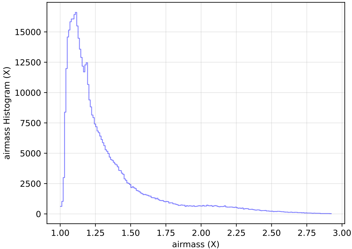
too_elab_heavy_r64_d2_griz_v3.4_10yrs All sky i band: airmass Histogram
