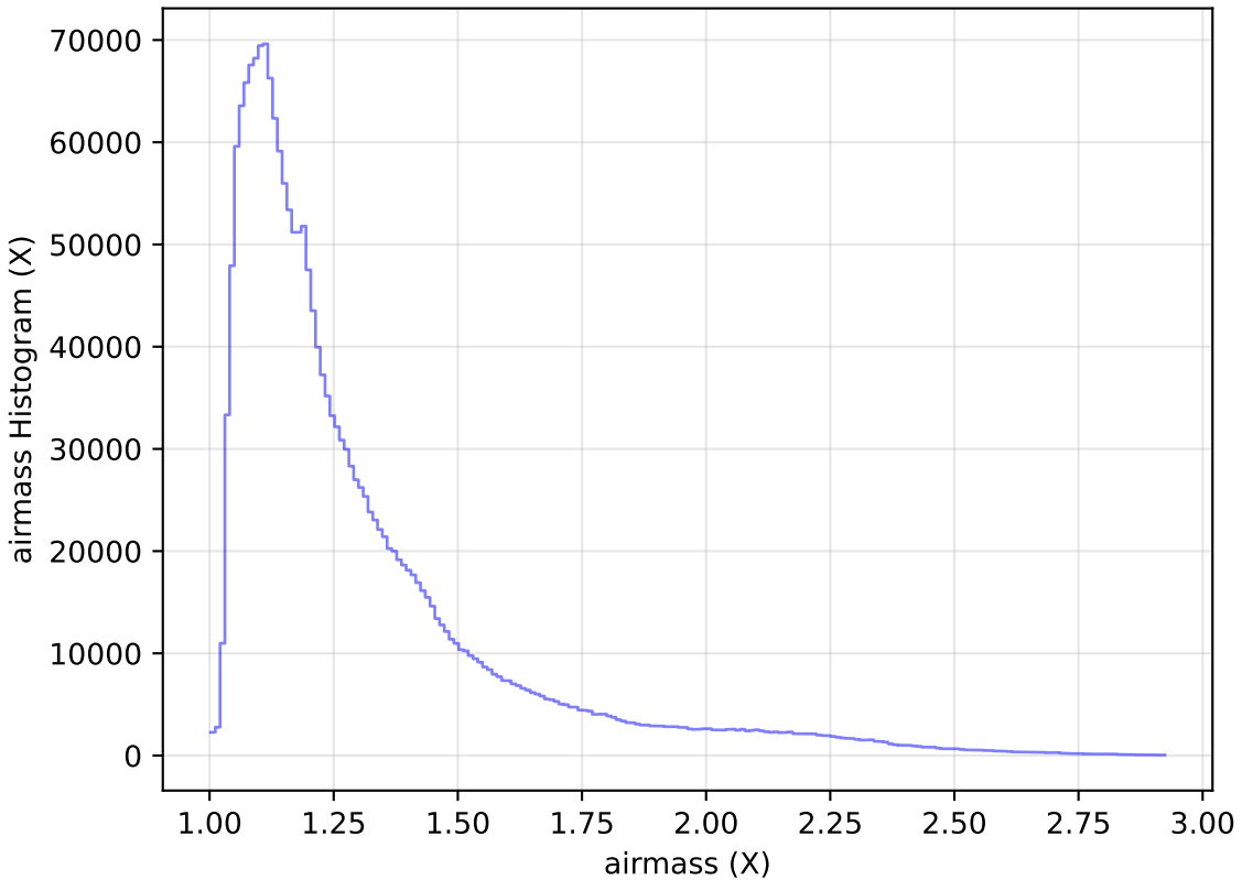
too_elab_heavy_r64_d2_griz_v3.4_10yrs All sky all bands: airmass Histogram
