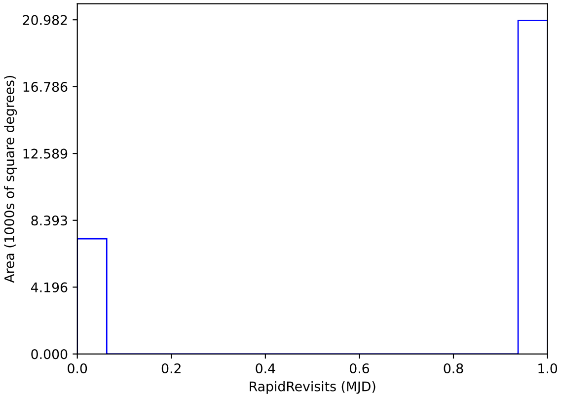
too_elab_heavy_r64_d2_griz_v3.4_10yrs All sky: RapidRevisits
