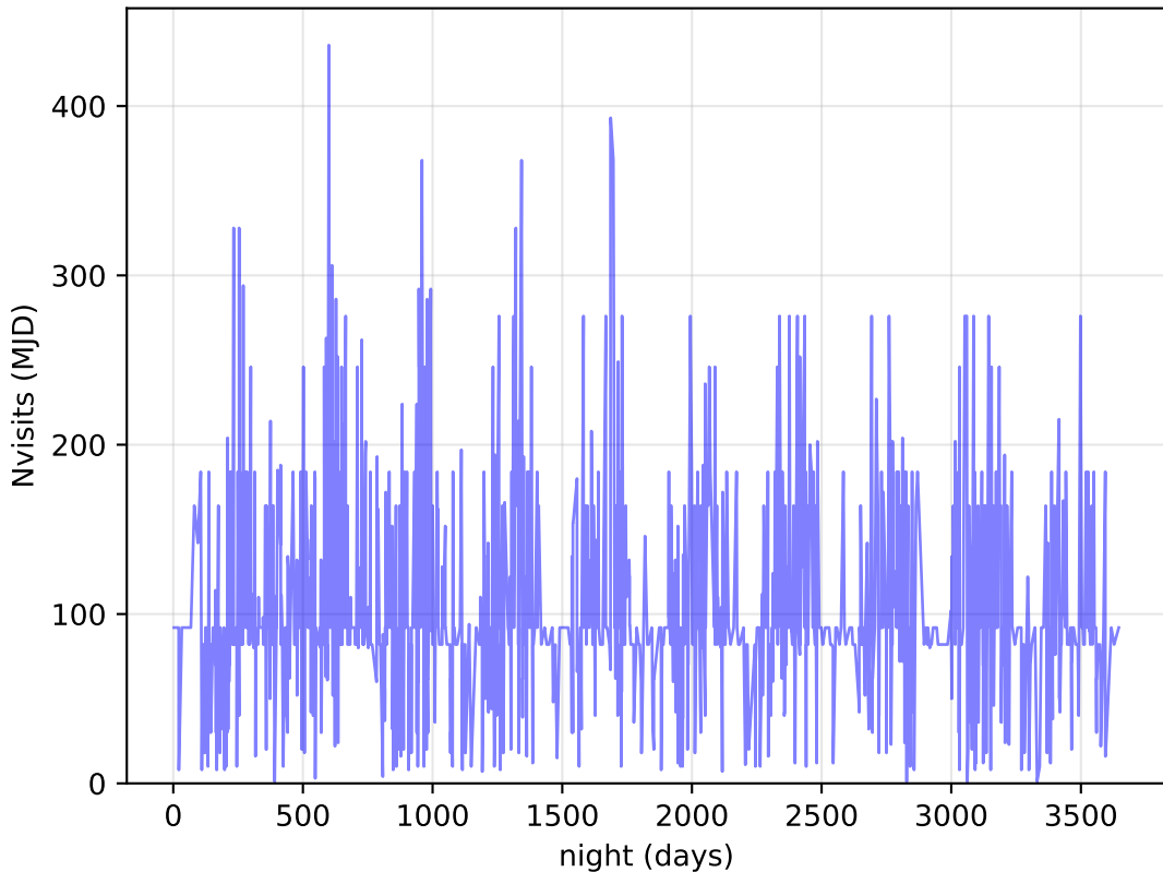
too_elab_heavy_r64_d2_griz_v3.4_10yrs DDF: Nvisits
