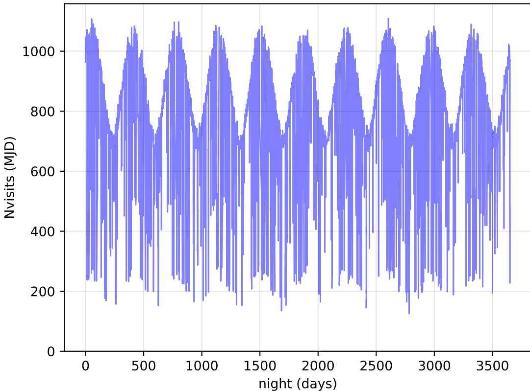
too_elab_heavy_r64_d2_griz_v3.4_10yrs All visits: Nvisits
