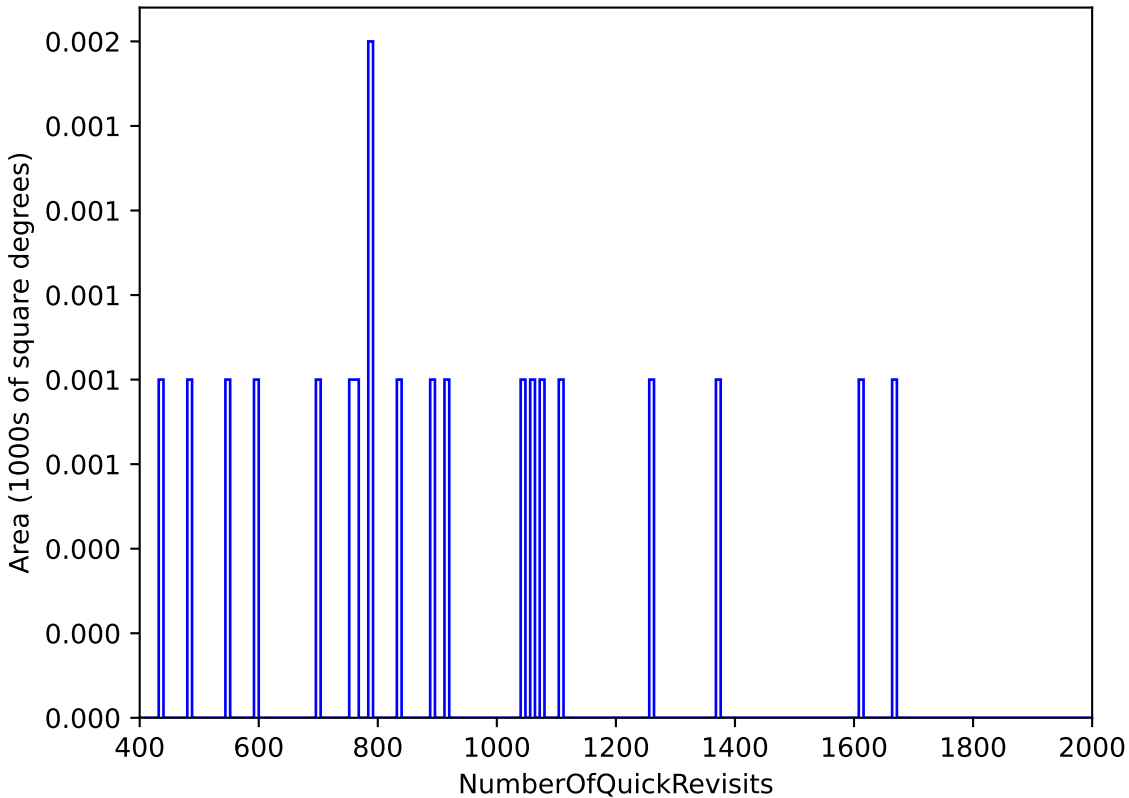
too_elab_heavy_r64_d2_griz_v3.4_10yrs WFD: NumberOfQuickRevisits
