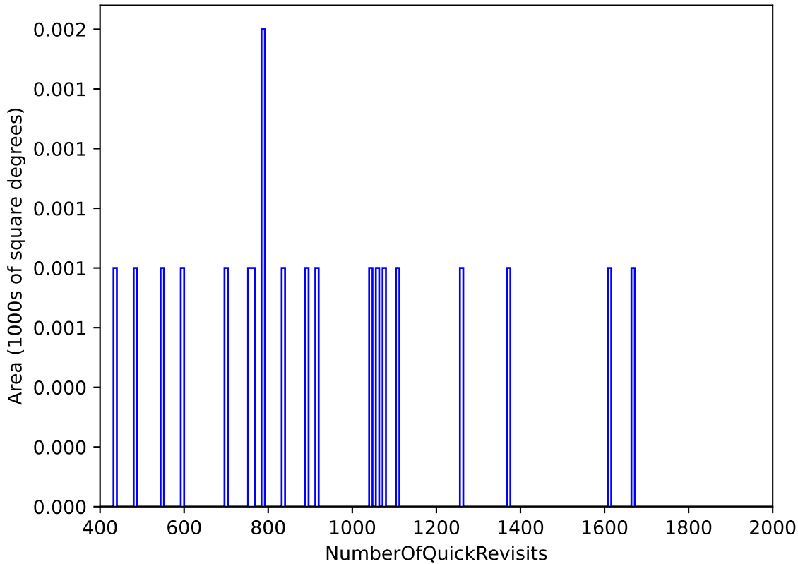
too_elab_heavy_r64_d2_griz_v3.4_10yrs All sky: NumberOfQuickRevisits
