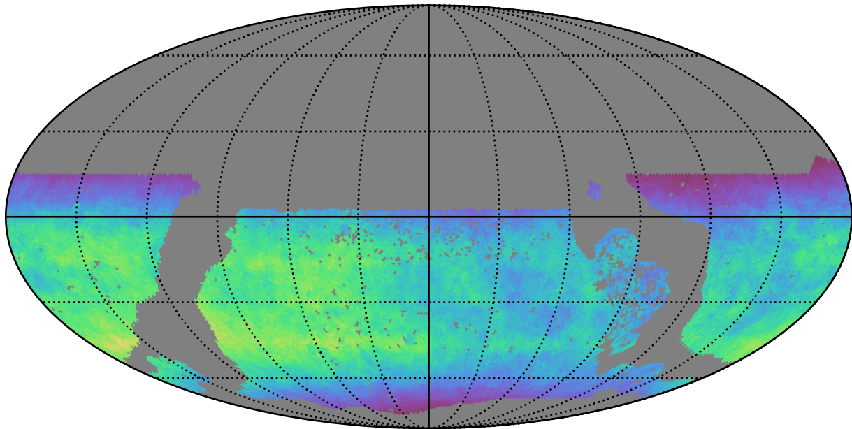
too_elab_heavy_r64_d2_griz_v3.4_10yrs WFD y band: Normalized Teff
